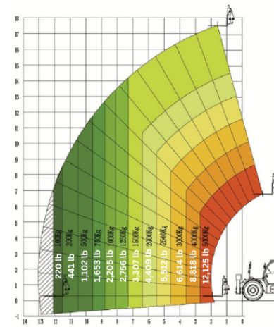
Outrigger Up
