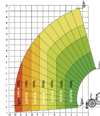
Outrigger Down
